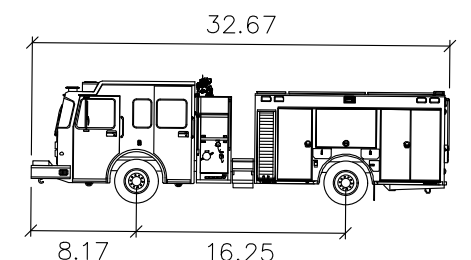
Toyne Pumper
