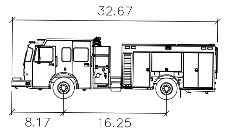
Toyne Pumper
