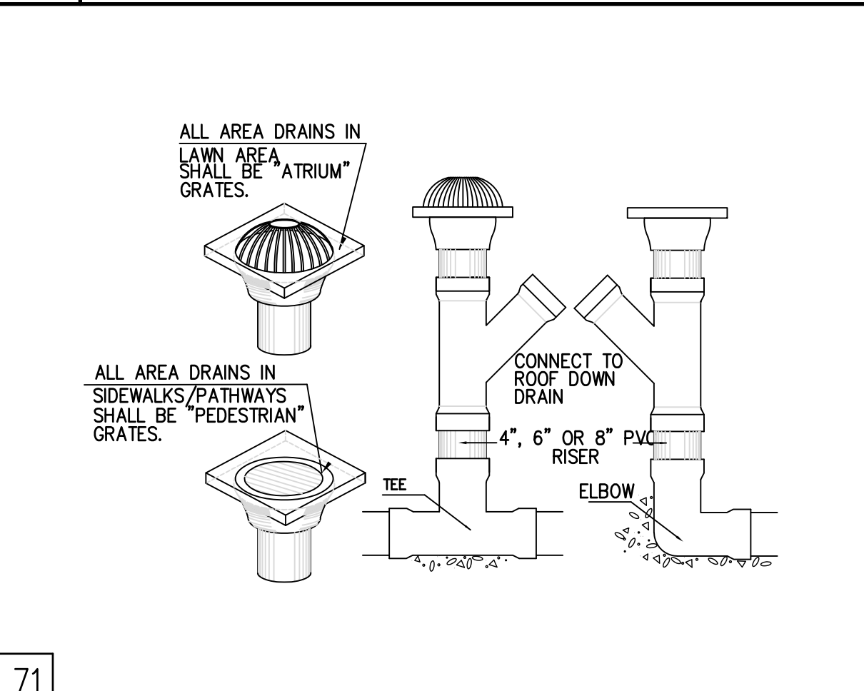
71 7 AREA DRAIN DETAIL
