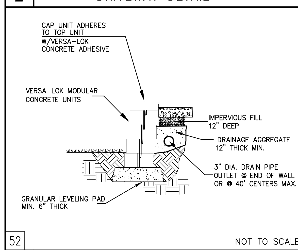
52 3 RETAINING WALL DETAIL
