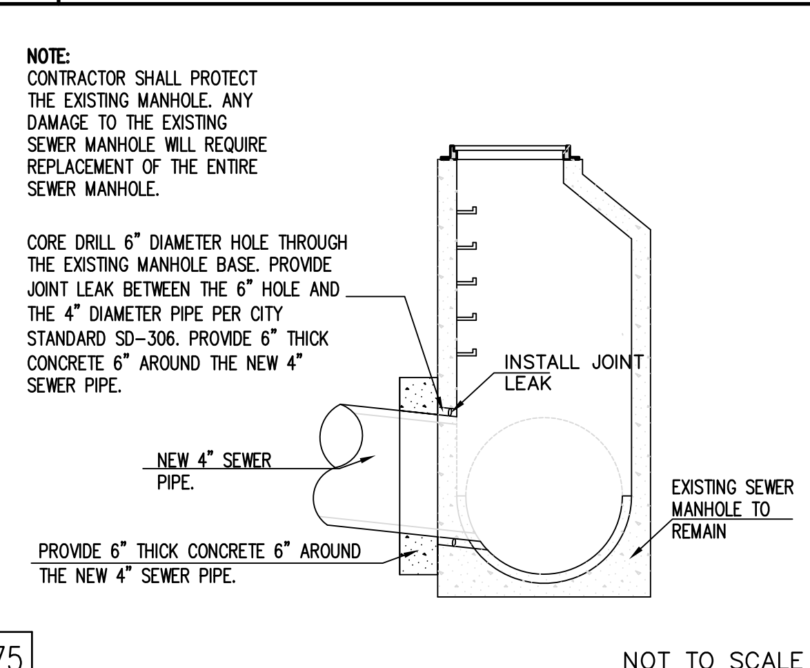
75 11 NEW PIPE TO MANHOLE DETAIL
