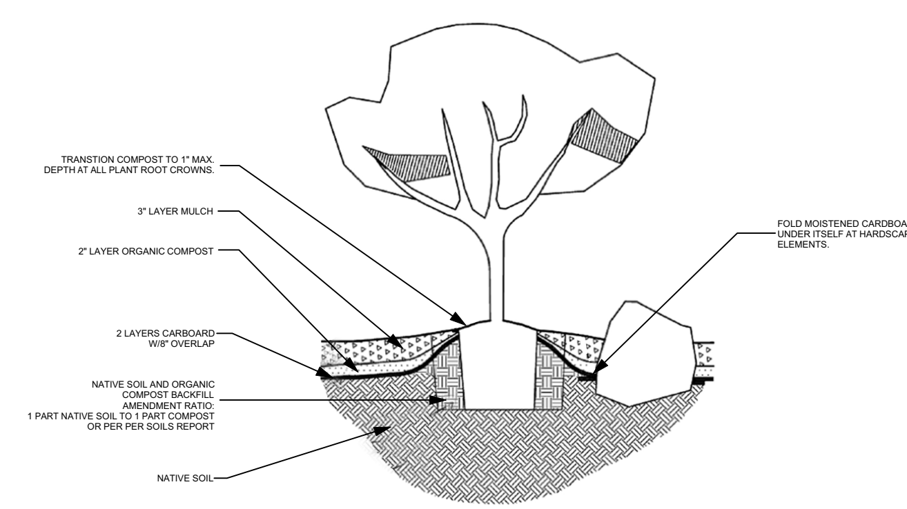
1 SHEET MULCH DETAIL
