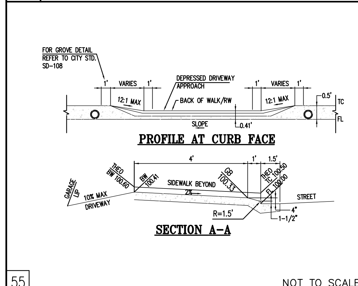
55 2 DRIVEWAY DETAIL
