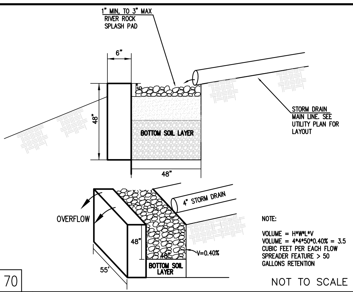
70 5 FLOW SPREADER DETAIL
