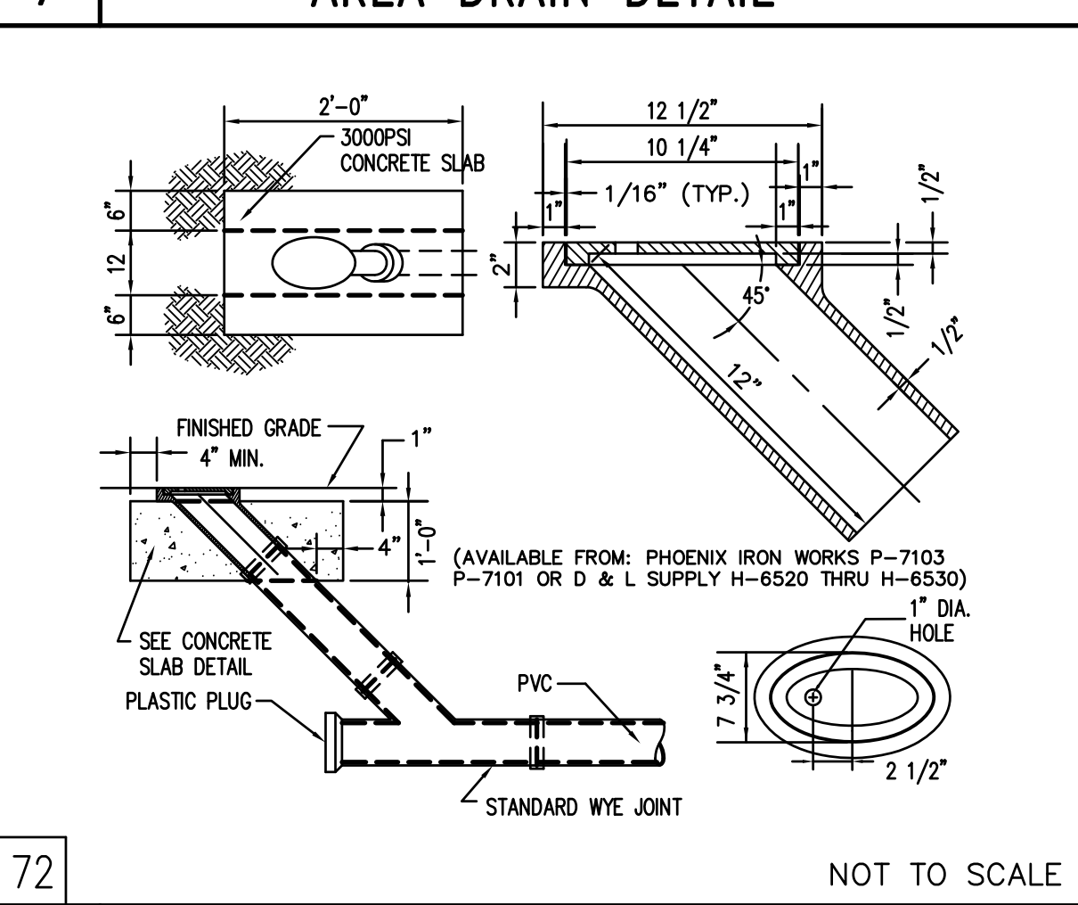
72 8 CLEANOUT AND GRATE DETAIL
