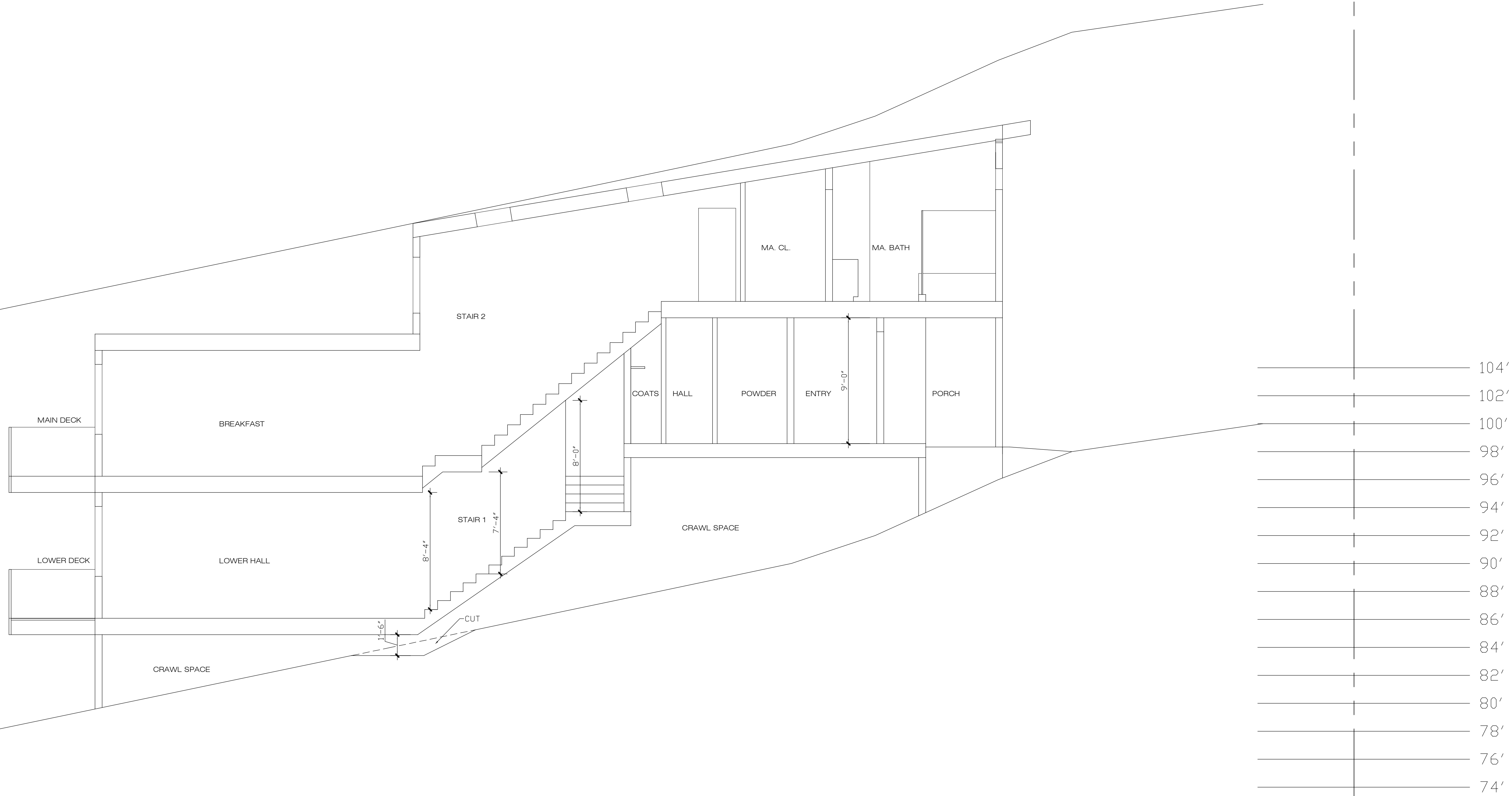
SECTION BB
