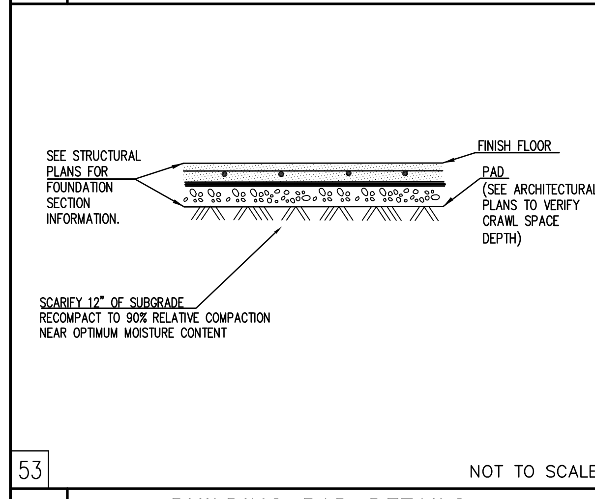
53 4 BUILDING PAD DETAILS
