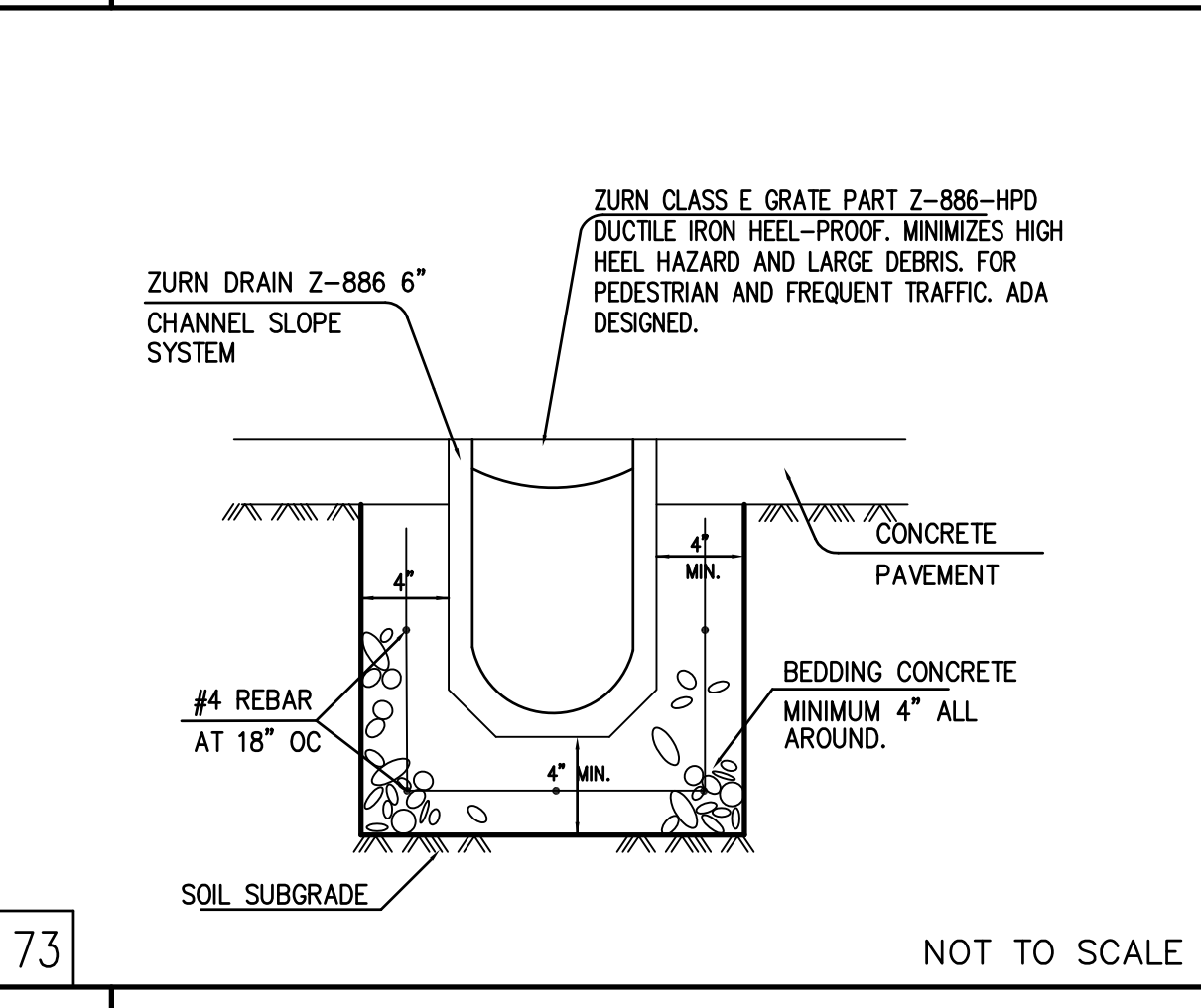
73 9 TRENCH DRAIN DETAILS
