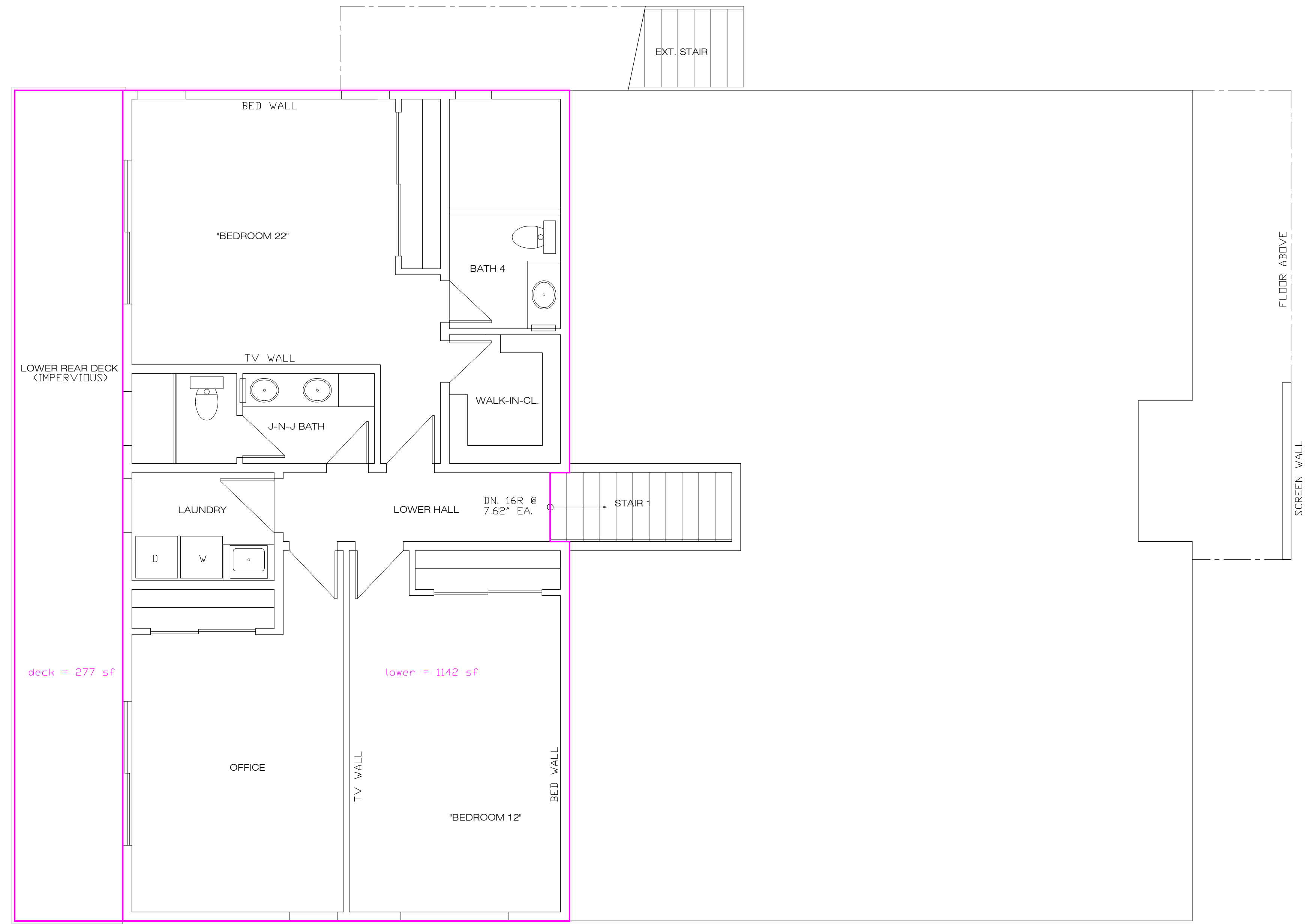
LOWER LEVEL FLOOR PLAN
