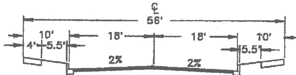
56' RESIDENTIAL - PUBLIC STREET (STANDARD WITH PLANTER STRIP)
