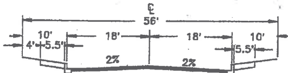
56' RESIDENTIAL - PUBLIC STREET (STANDARD WITHOUT PLANTER STRIP)
