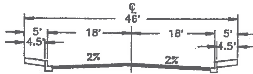
46' RESIDENTIAL - PUBLIC STREET (MINIMUM STANDARD WITH P.U.E.)
