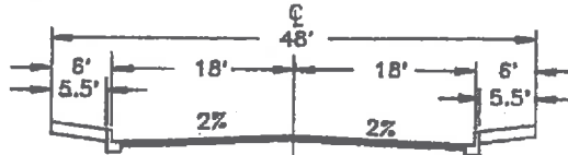
48' RESIDENTIAL - PUBLIC STREET (MINIMUM STANDARD WITHOUT P.U.E.)
