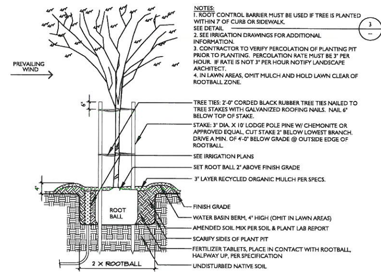
1 TREE STAKING DETAIL - ON SITE SCALE: 3/8" = 1'-0"
