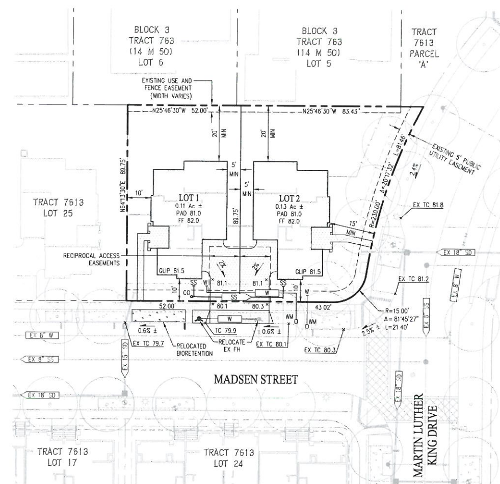
SITE/GRADING/UTILITY PLAN
