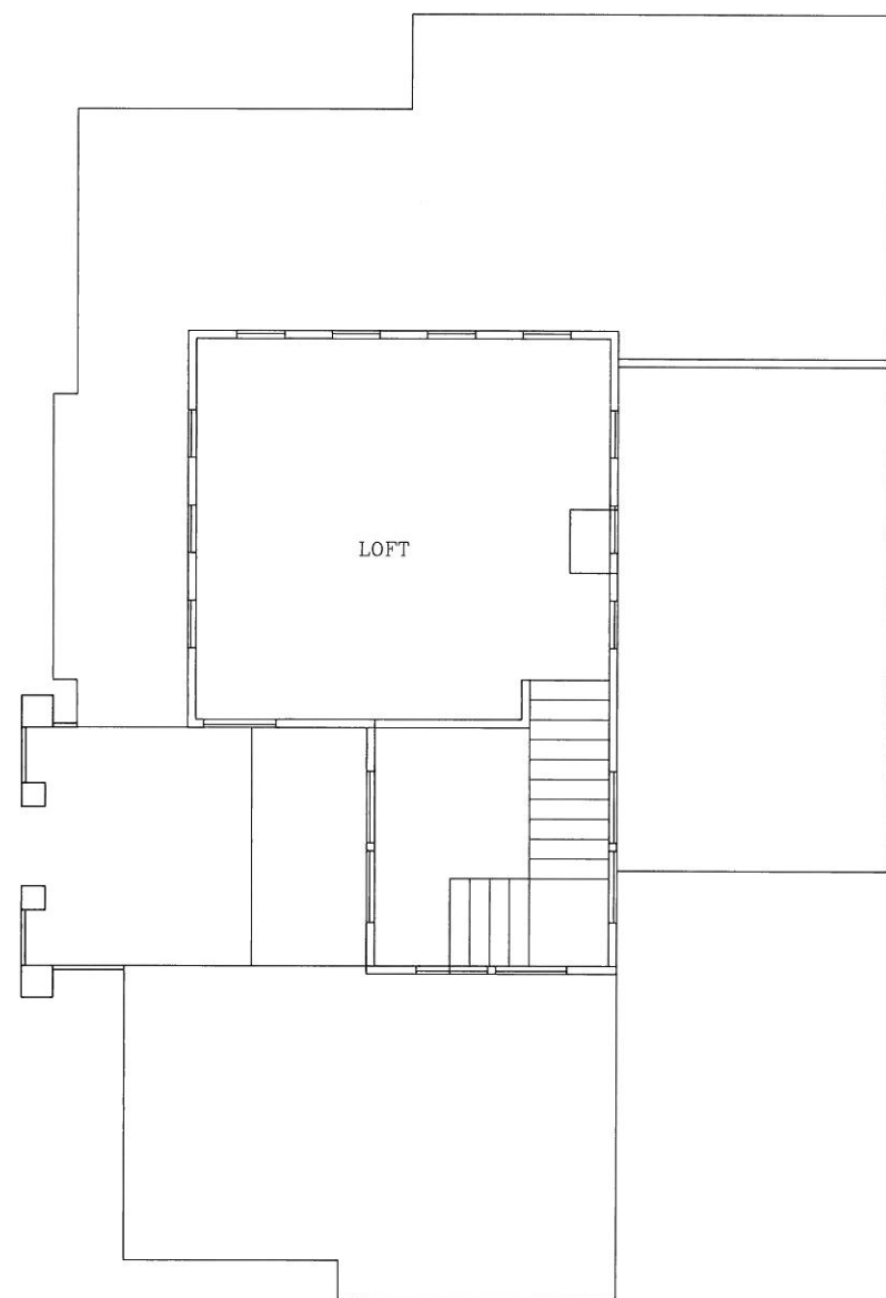
THIRD FLOOR (LOFT) PLAN SCALE: 1/4" = 1'-0"
