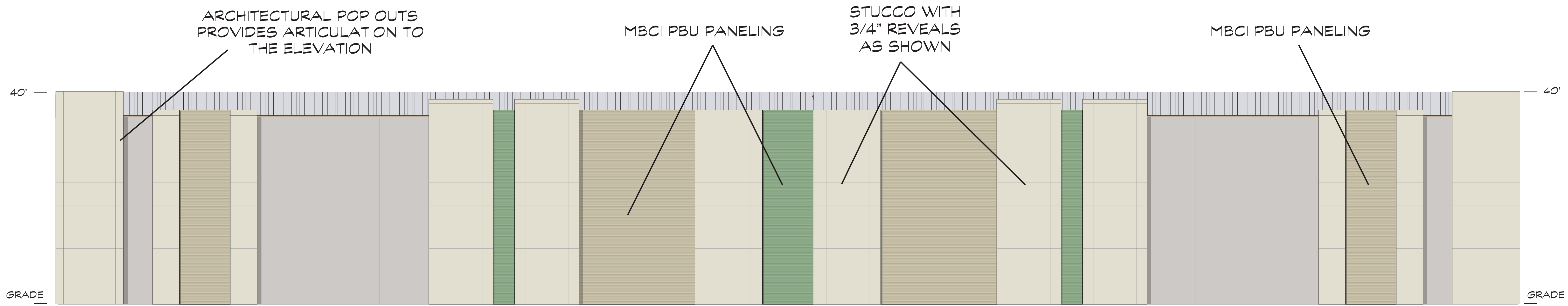
South Elevation
