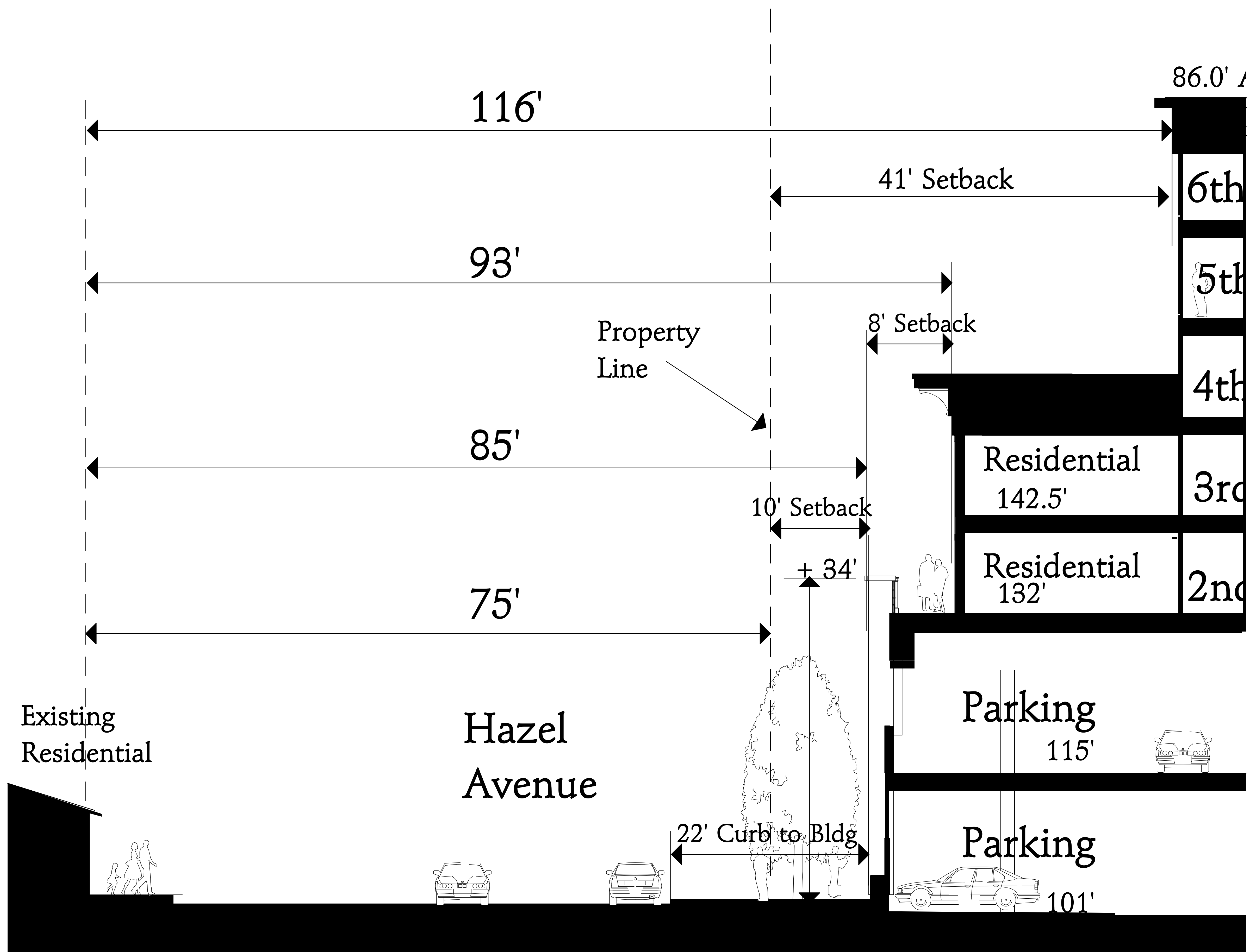
Section A1 @ Hazel Avenue 3/16" = 1'-0"
