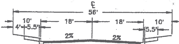
56' RESIDENTIAL - PUBLIC STREET (STANDARD WITHOUT PLANTER STRIP)
