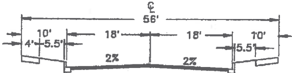
56' RESIDENTIAL - PUBLIC STREET (STANDARD WITH PLANTER STRIP)
