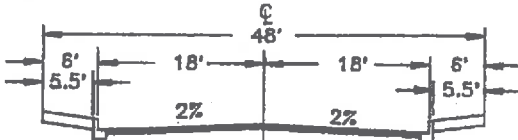
48' RESIDENTIAL - PUBLIC STREET (MINIMUM STANDARD WITHOUT P.U.E.)
