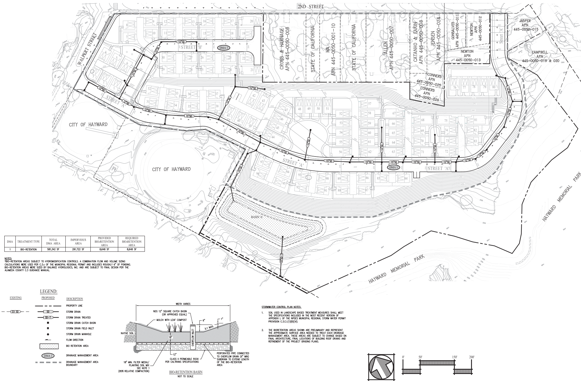
STORMWATER MANAGEMENT PLAN FIGURE 6
