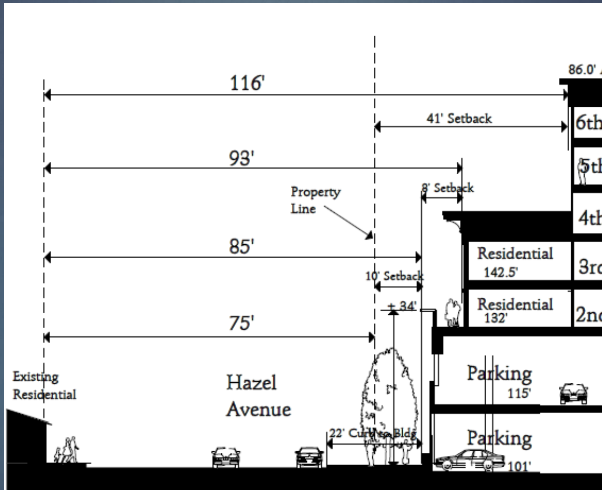
Section A1 @ Hazel Avenue
