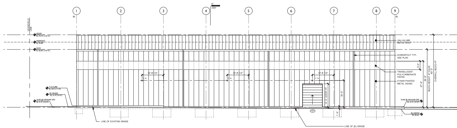
02-WEST ELEVATION
